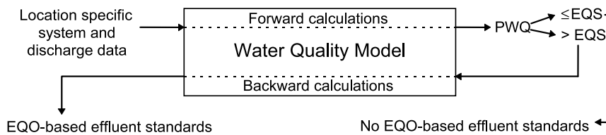
Figure 3 Schematic presentation of an immission assessment procedure (PWQ = predicted water quality, EQS = environmental quality standard)
